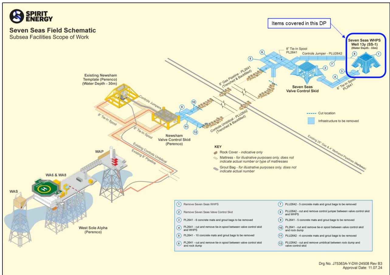
Figure 1.6.2: Seven Seas Facilities Schematic Seven Seas Wellhead Protection Structure Decommissioning Programme Page 10 of 31
