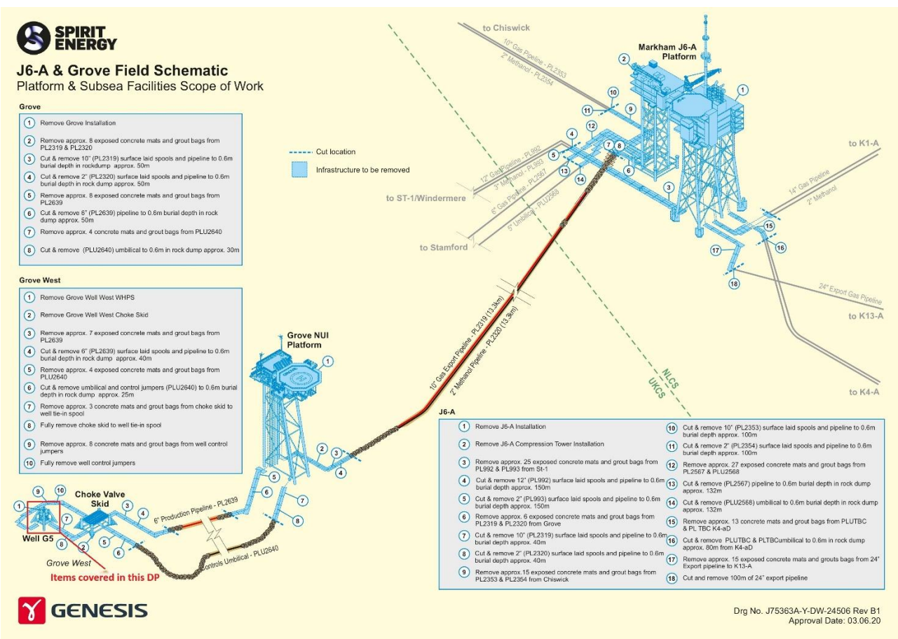
Figure 1.6.2 Grove G5 Facilities Schematic
